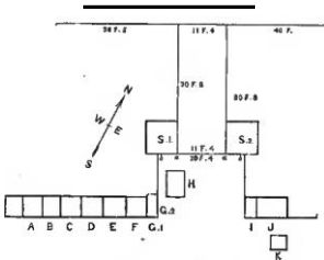
Plan of ancient building at Euyuk.
