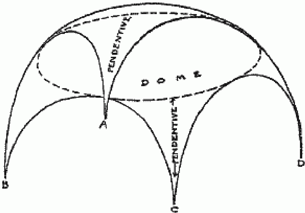
Fig. 8.—The Saucer Dome Or Dome-Vault.
