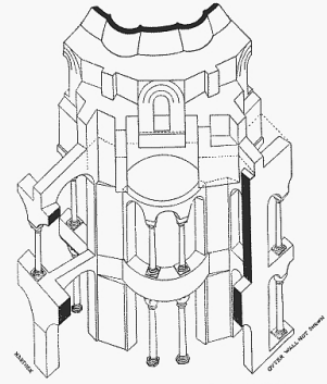
THE REAR - WITH GYMNASIUM FLOOR & REAR REMOVED CONSTRUCTIVE SECTIONS OF THE SOUTH WEST EXEDRA
