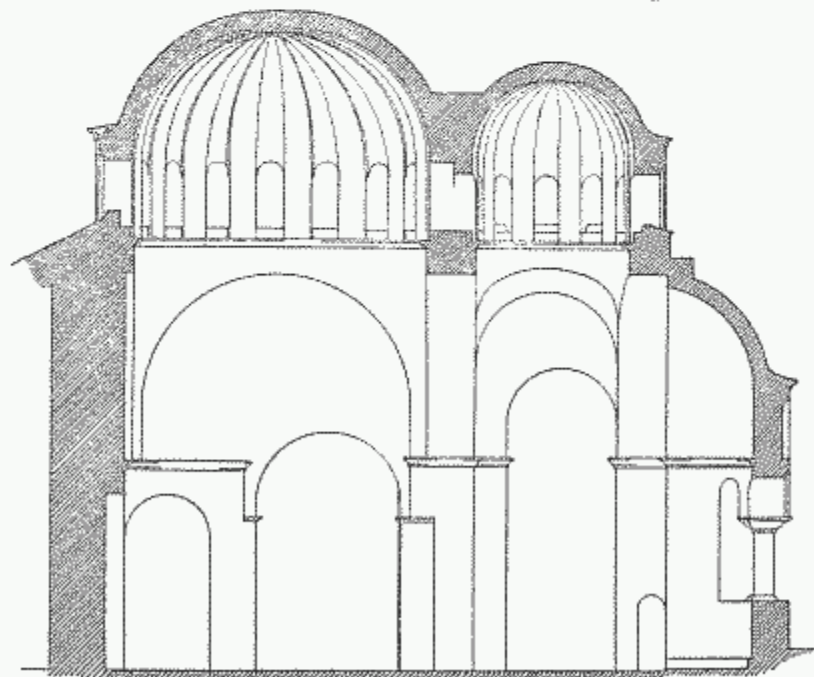
LONGITUDINAL SECTION THROUGH MIDDLE CHURCH
