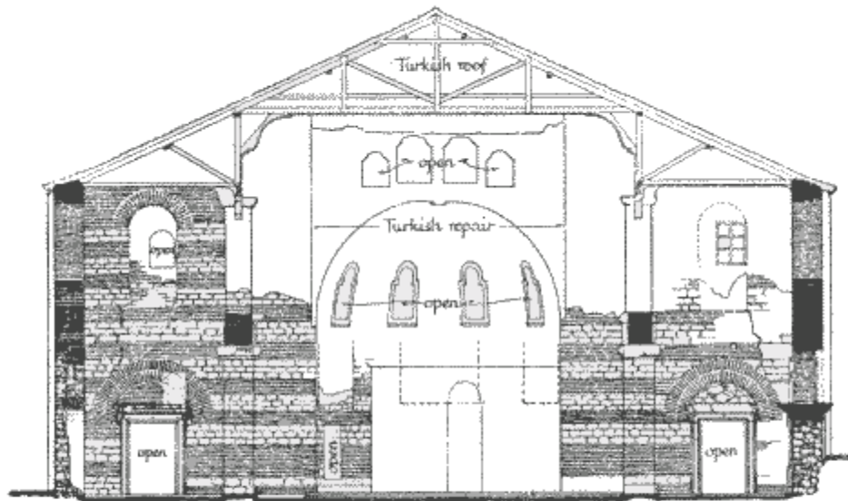
CROSS SECTION LOOKING EAST
