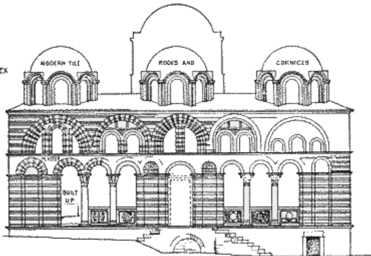
FRONT ELEVATION
