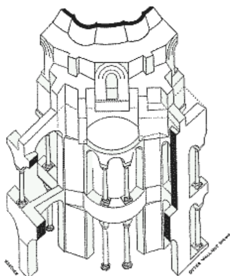
THE REAR - WITH GYMNASION FLOOR & REEF REMOVED CONSTRUCTING SECTIONS OF THE SOUTH WEST EXEDRA
