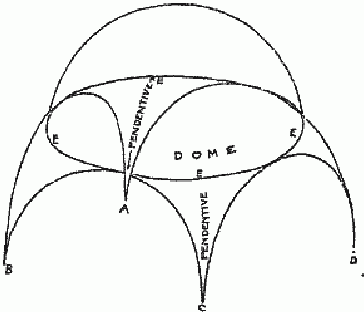
Fig. 9.—The Dome on Pendentives.
