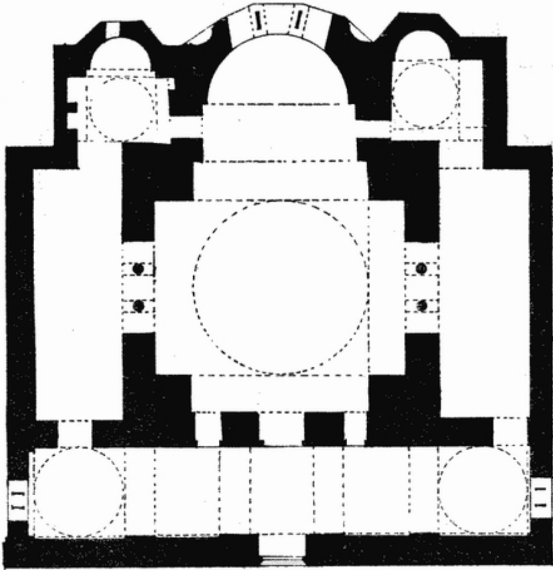
Fig. 102.—S. Saviour in the Chora (restored plan).
