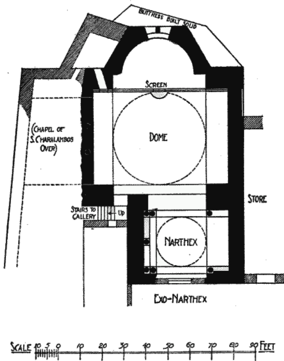
Fig. 104.—Church of the Archangels at Sygé.
