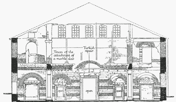
CROSS SECTION LOOKING WEST
