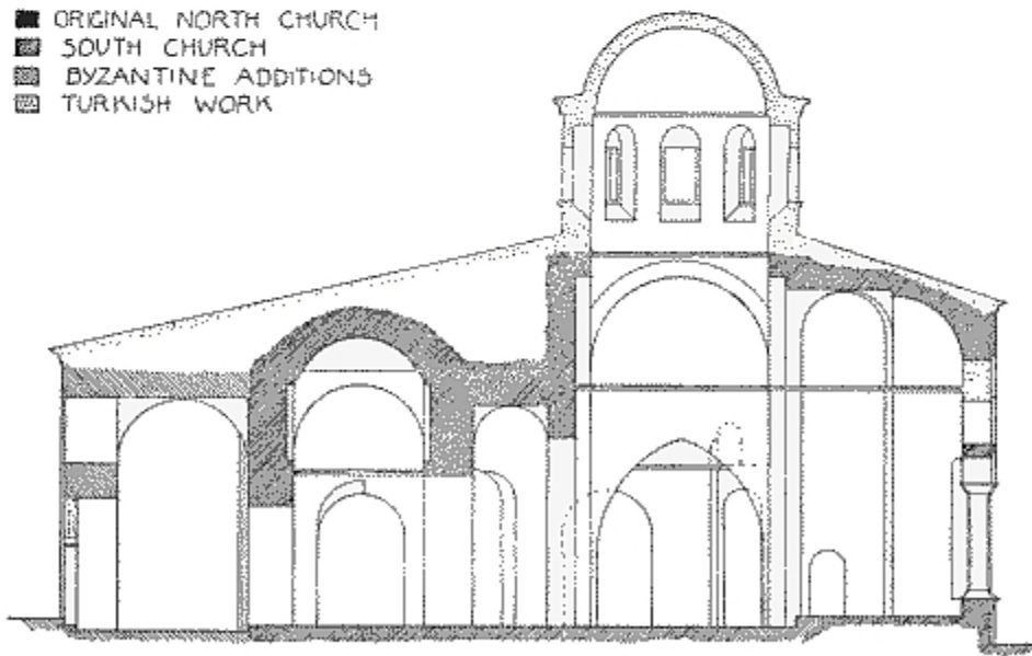
SECTION THROUGH SOUTH CHURCH
