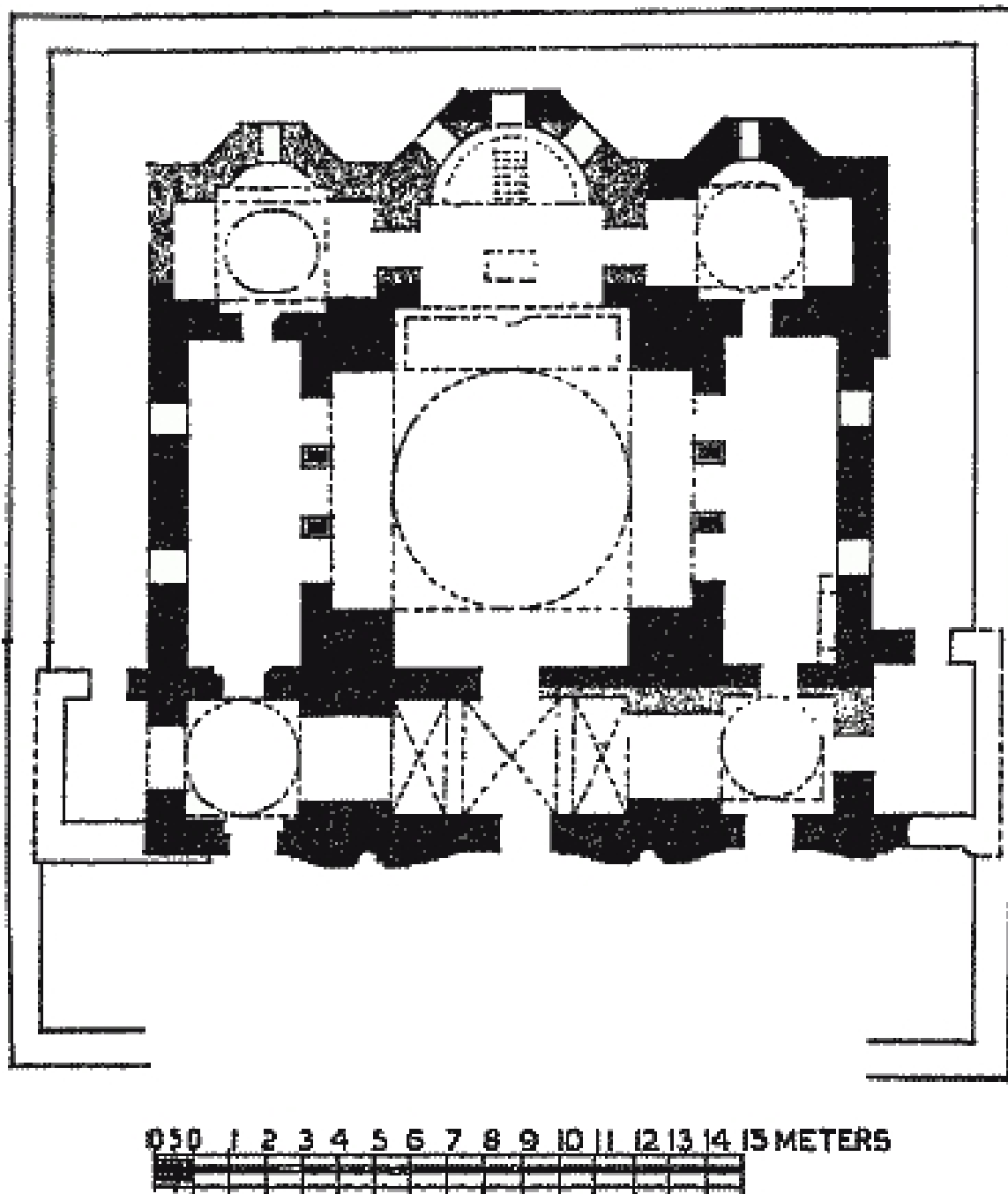
Fig. 5.—The Church of the Koimesis, Nicaea (Wulf).
