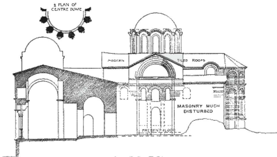
SOUTH ELEVATION AND SECTION THRO' VAULTED BAY OF NARTHEX
