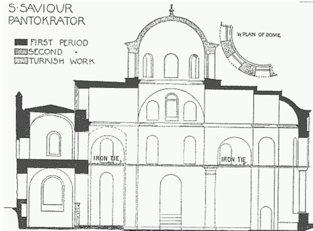
LONGITUDINAL SECTION THROUGH NORTH CHURCH
