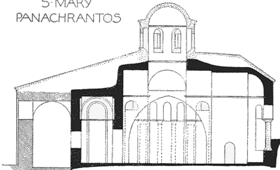
SECTION THROUGH NORTH CHURCH
