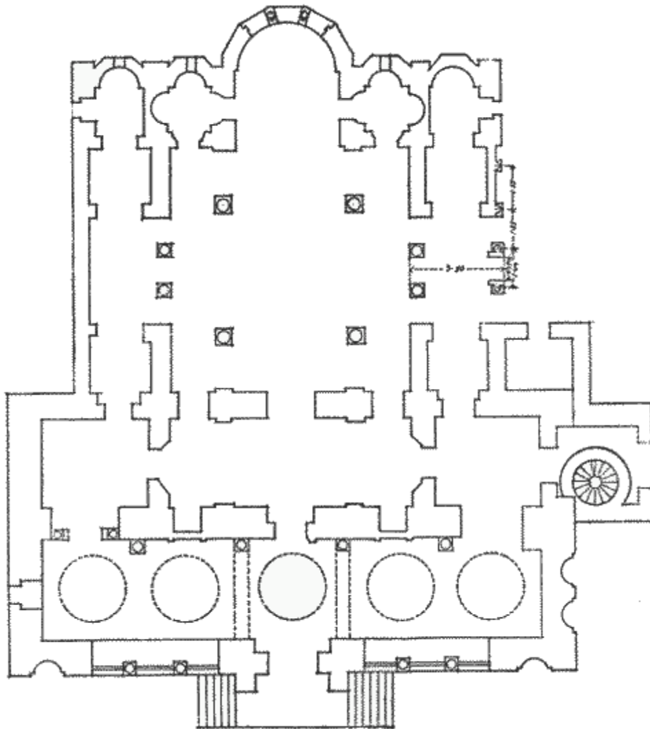
Fig. 82.—S. Theodore. Plan as given by Texier
