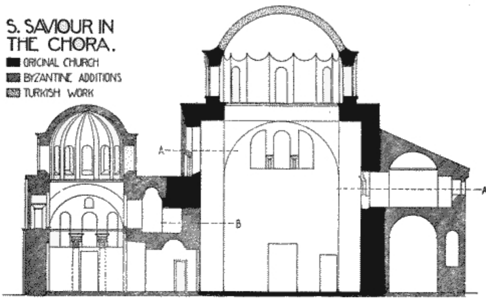
CROSS SECTION LOOKING WEST
