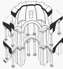
THE INTERIOR ARRANGEMENT SHOWING GYMNASIUM FLOOR, VAULTING ROOF AND SPRINGING OF DOME
