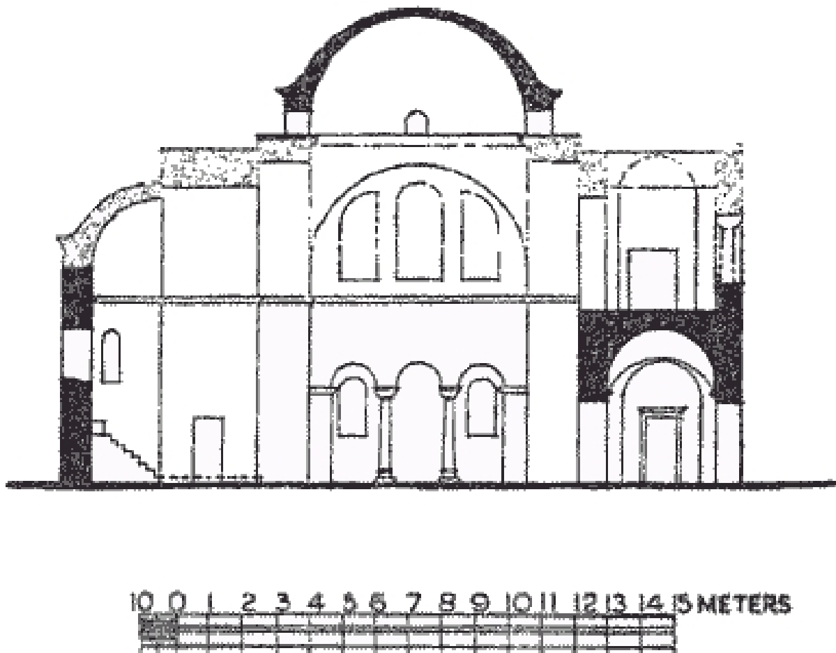
Fig. 6.—The Church of the Koimesis, Nicaea (Rott).
