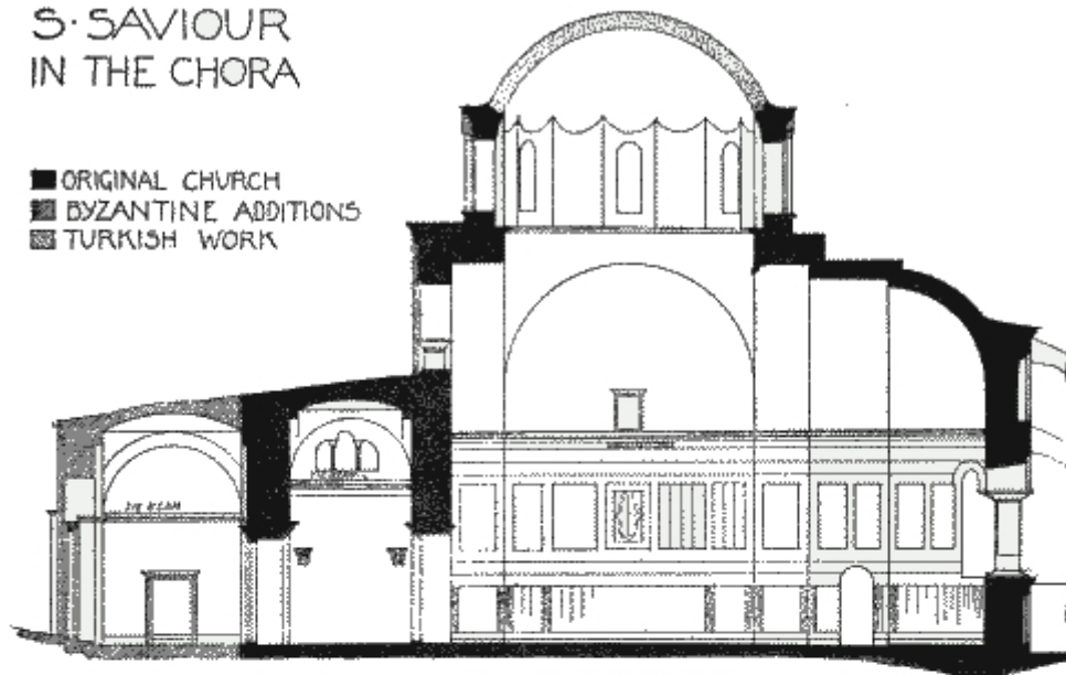
SECTION THROUGH THE CHURCH
