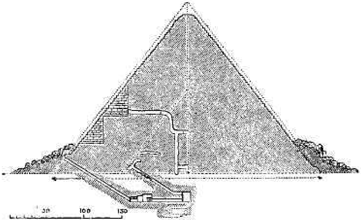
SECTION OF THE THIRD PYRAMID, SHOWING PASSAGES.
